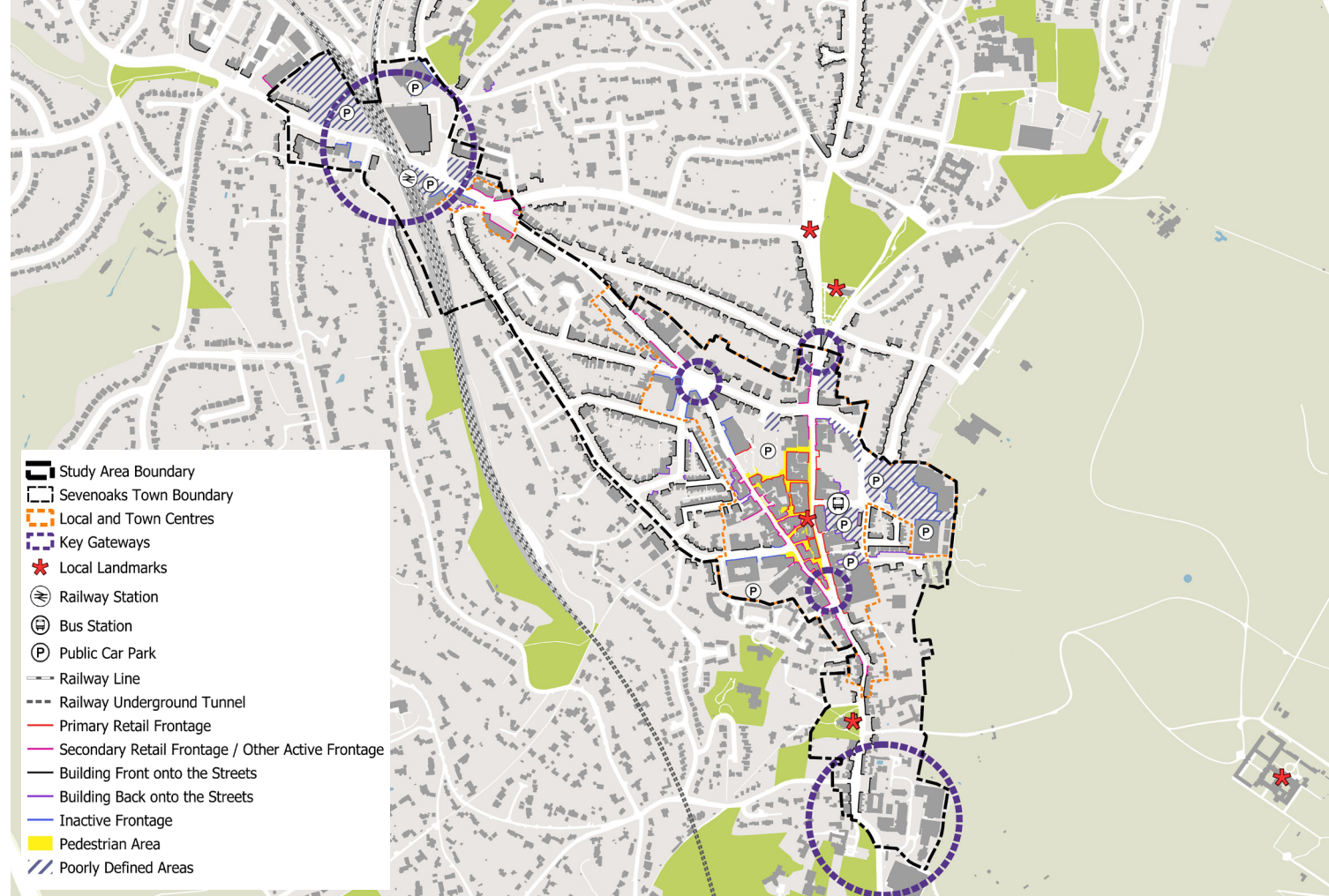
Figure 2.4: Townscape plan
